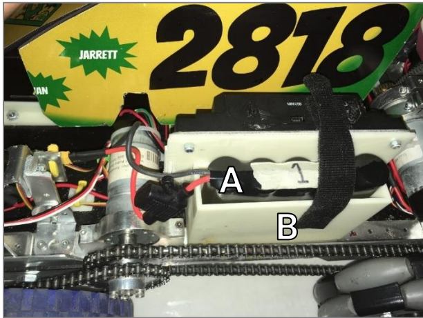
Figure 20: Battery Security
