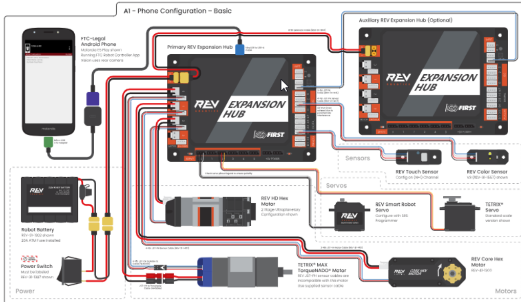
Figure 1: Smartphone/Expansion Hub Configuration
