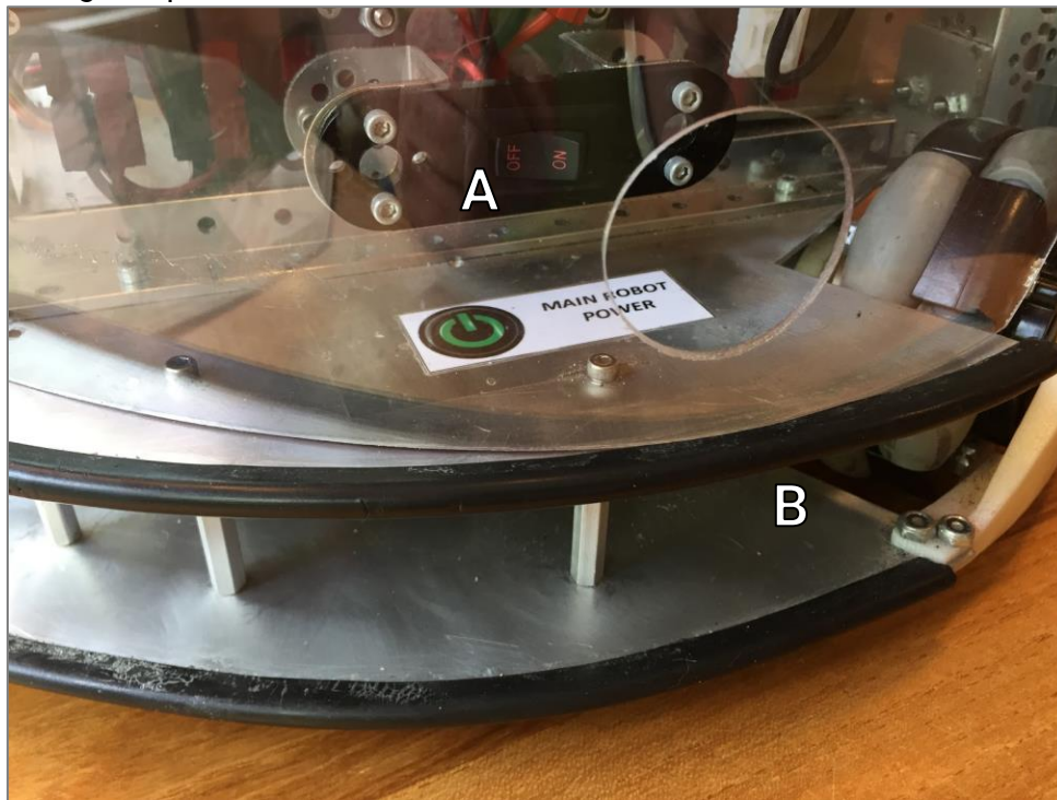
Figure 21: Power Switch Placement, Side Shield and Chassis Insulation
