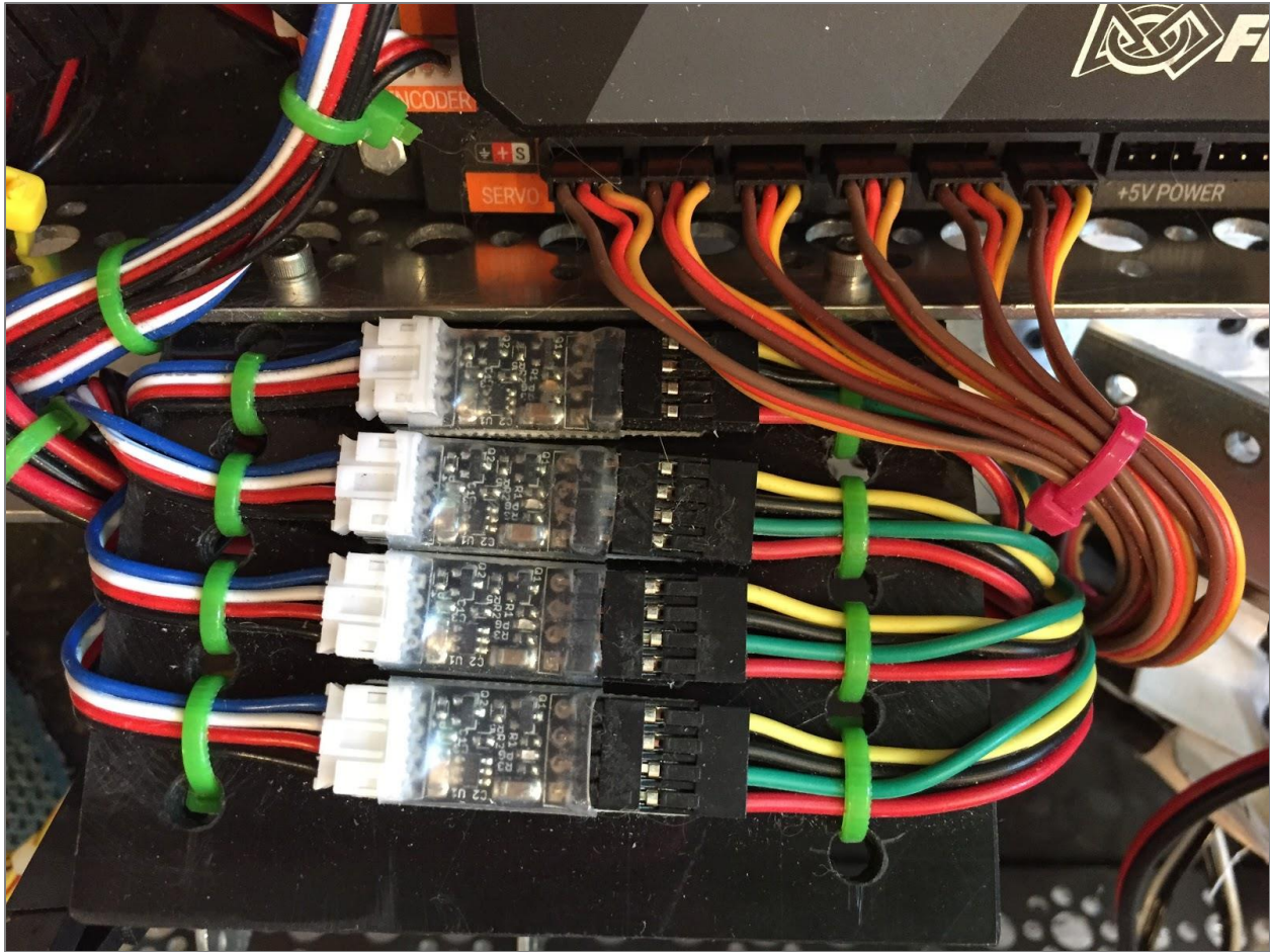
Figure 38: Level Shifters
