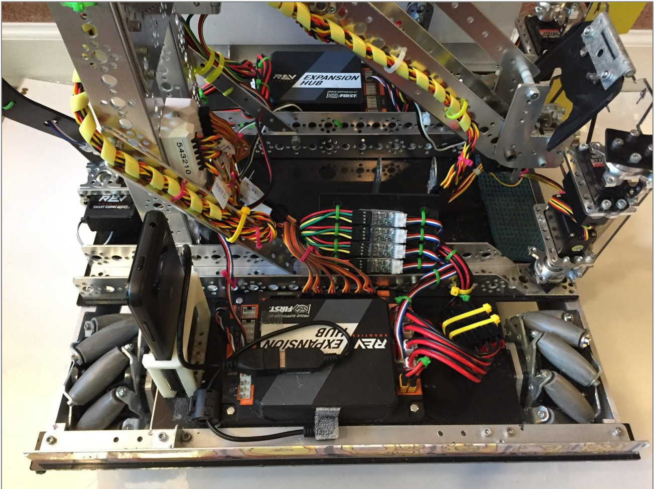
Figure 17: Multiple Wire Management Types
