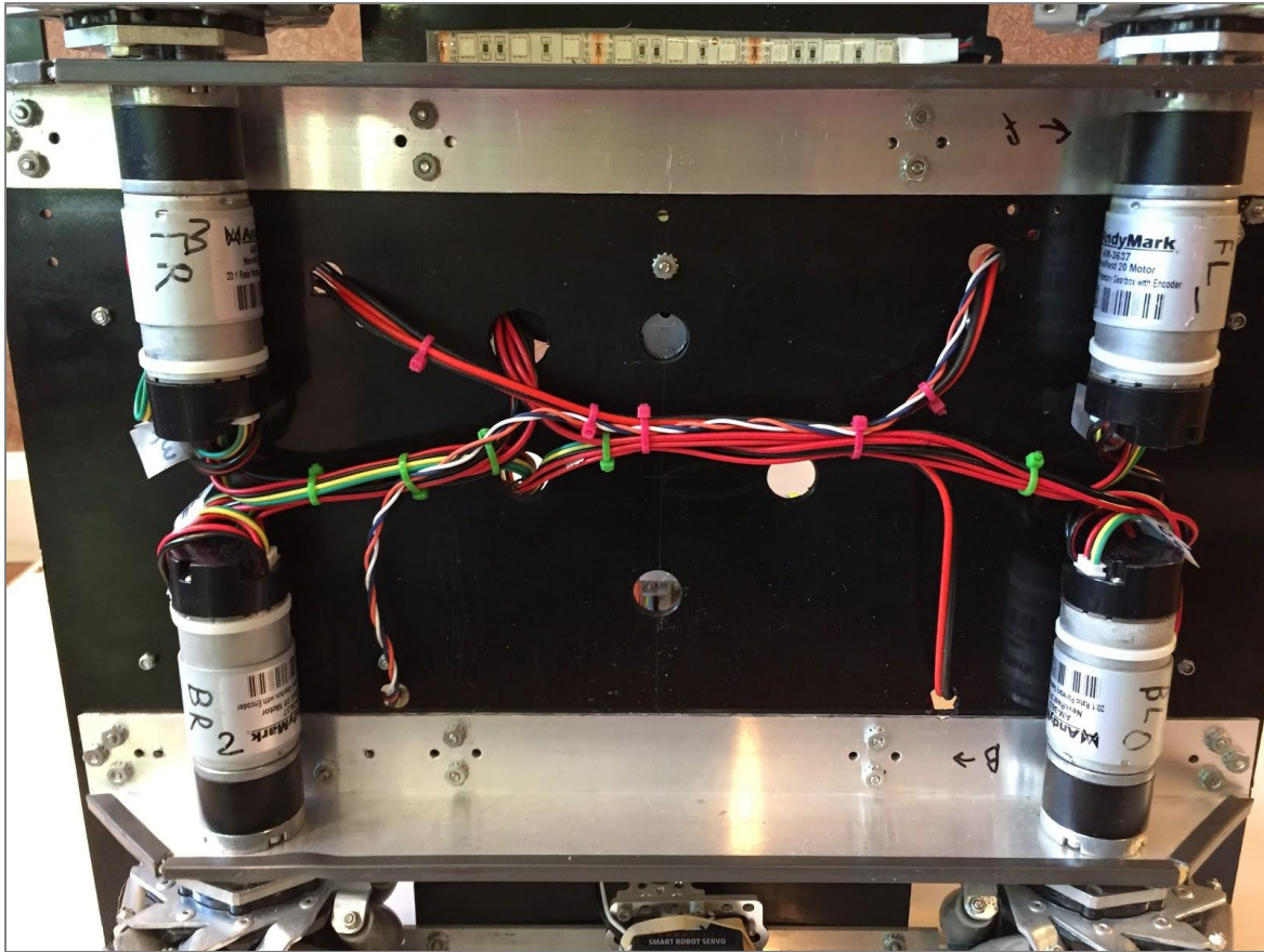
Figure 11: Securing Wires
