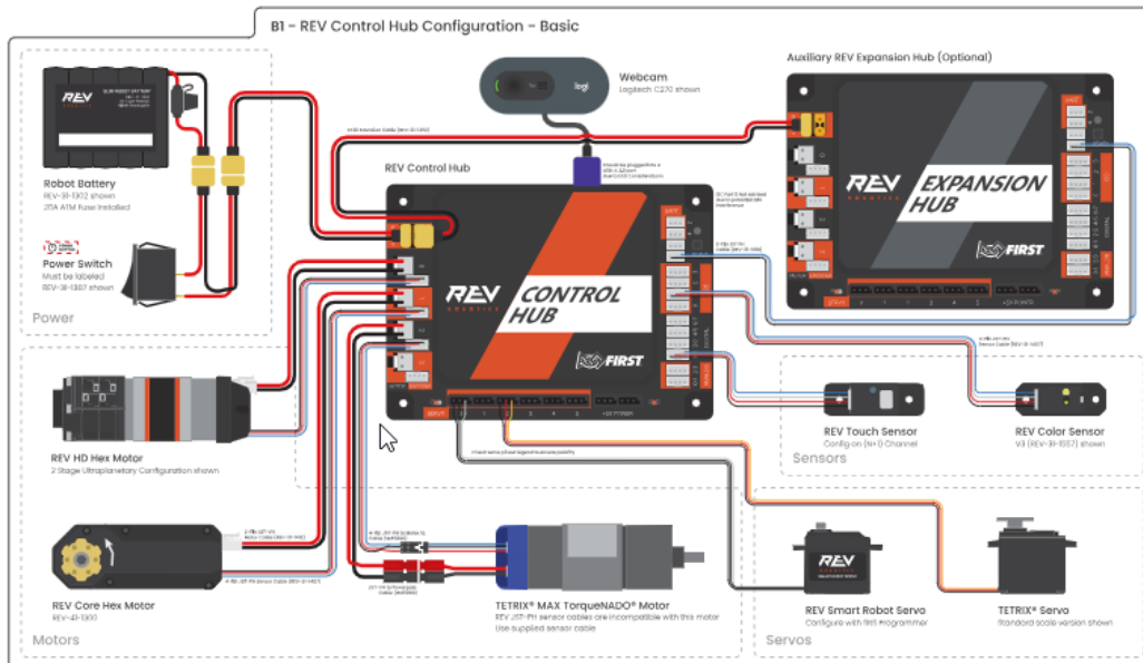
Figure 2: Control Hub/Expansion Hub Configuration
