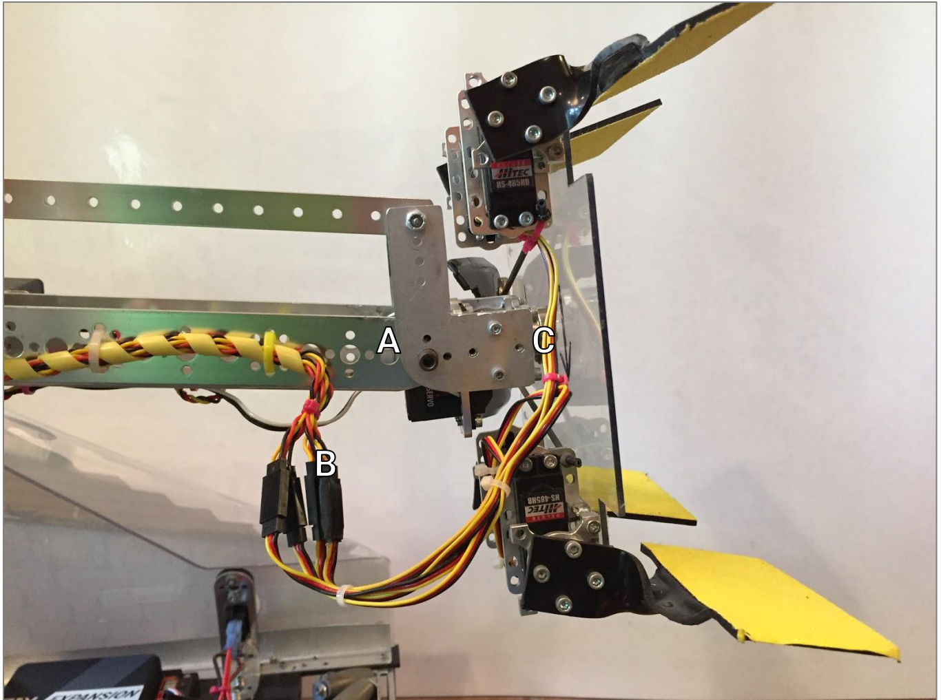
Figure 12: In-Line Connections
