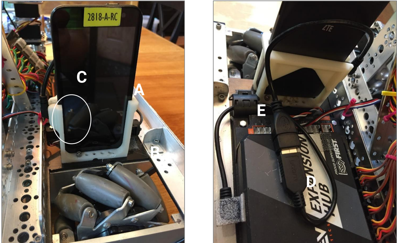
Figure 24: Phone Mounting
