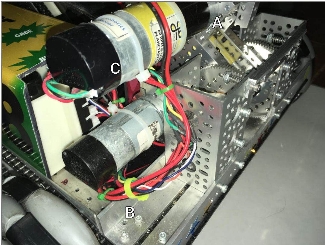
Figure 19: Wires Near Moving Parts
