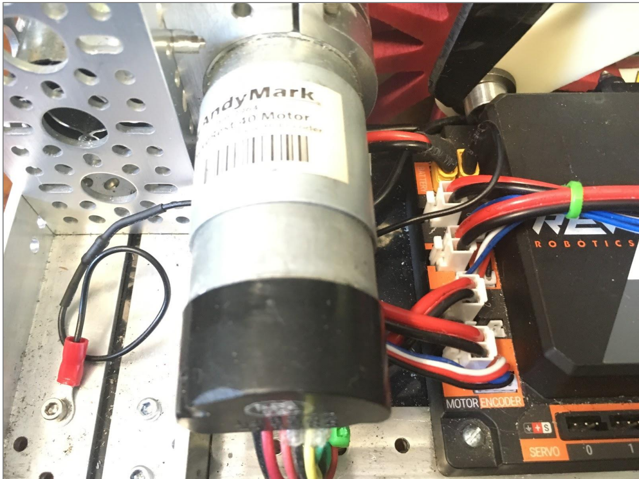
Figure 26: Grounding Strap
