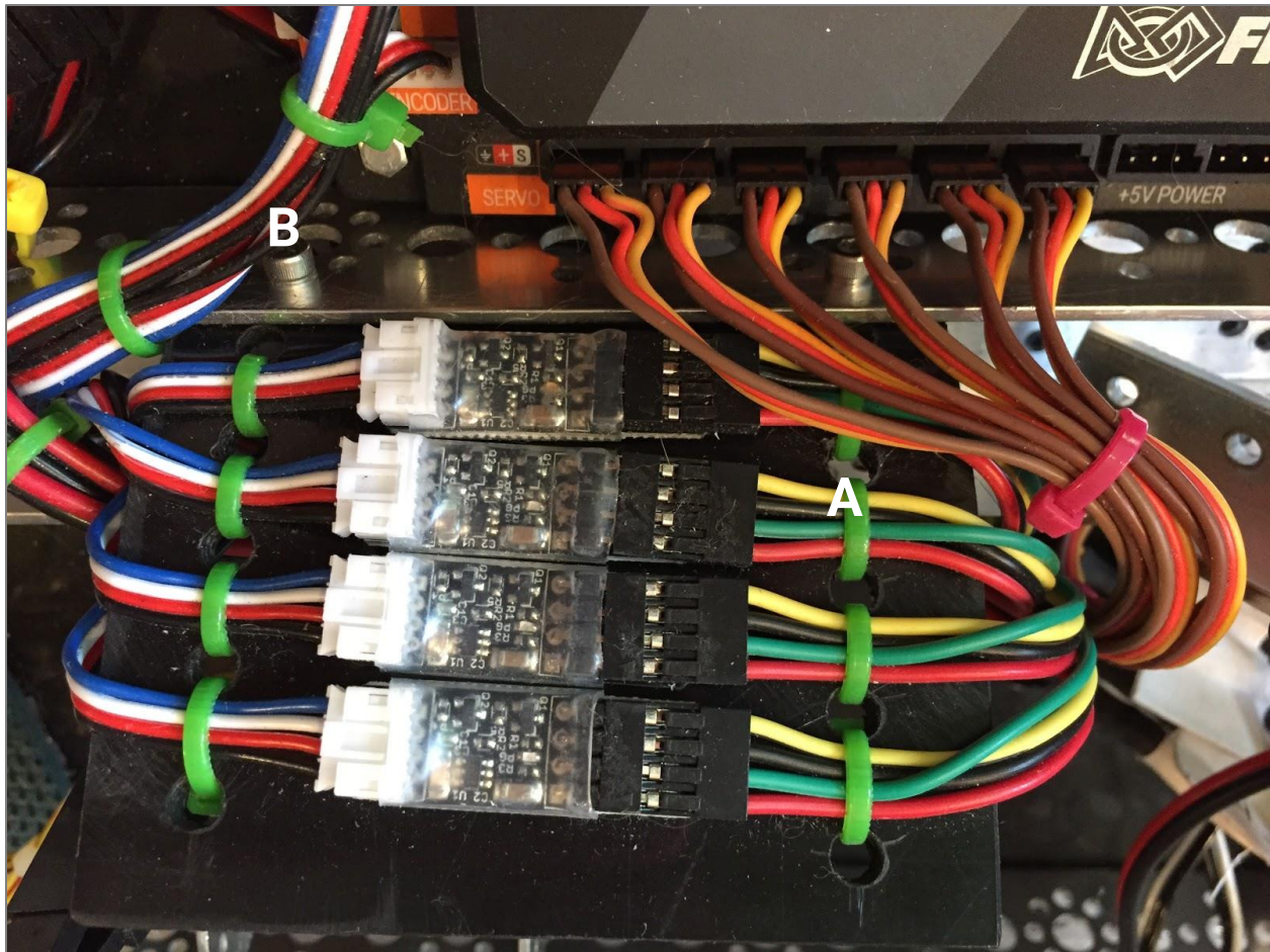
Figure 28: Level Shifters
