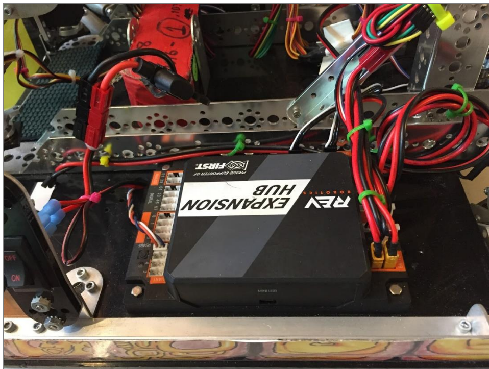
Figure 10: Strain Relief and Wire Restraints
